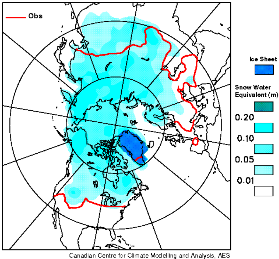
Figure 5.2: Mean December/January/February snow water equivalent (m) produced by the CCCMA global coupled model, compared with the snow extent derived from the USAF global climatology (Foster and Davey, 1988) (red line). Courtesy of G. Flato, CCCMA.
