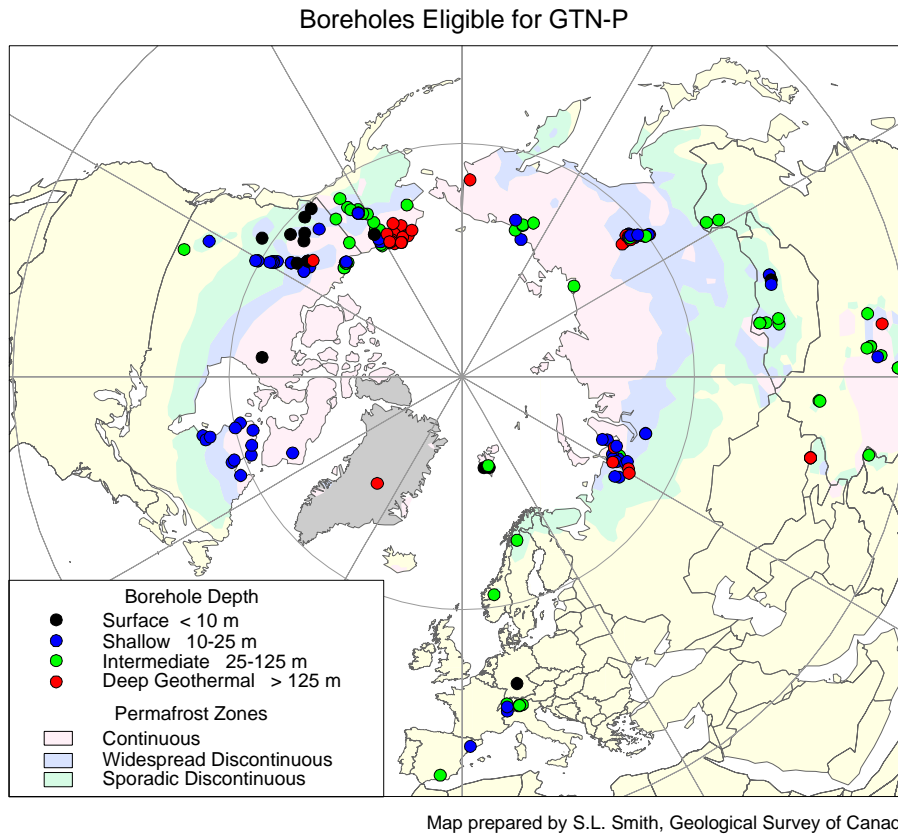
Figure 5.3: Distribution of Northern Hemisphere permafrost zones (Brown et al., 1997) and the proposed distribution of borehole sites for the Global Terrestrial Network for Permafrost. Courtesy of M. Burgess, Geological Survey of Canada.
